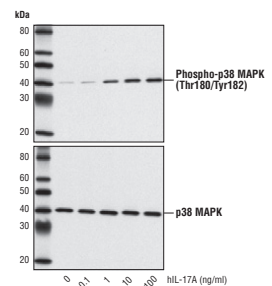
Human foreskin fibroblasts treated with hIL-17A for 15 minutes were examined using phospho- and total p38 MAPK antibodies.
