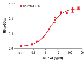
The production of IL-6 by human foreskin fibroblasts cultured with increasing concentrations of hIL-17A for 48 hours was assessed.
