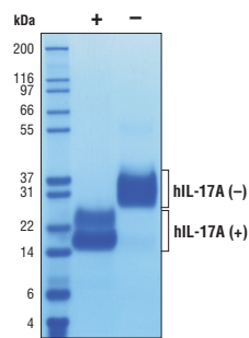
6 μg reduced (+) and non-reduced (-) recombinant hIL-17A.
