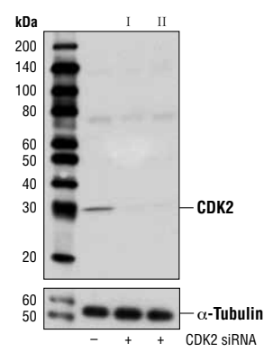
Western blot analysis of extracts from HeLa cells, transfected with 100 nM SignalSilence® Control siRNA (Unconjugated) #6568 (-), SignalSilence® CDK2 siRNA I #8618 (+) or SignalSilence® CDK2 siRNA II (+), using CDK2 (78B2) Rabbit mAb #2546 (upper) or \alpha -Tubulin (11H10) Rabbit mAb #2125 (lower). The CDK2 (78B2) Rabbit mAb confirms silencing of CDK2 expression, while the \alpha -Tubulin (11H10) Rabbit mAb is used as a loading control.
