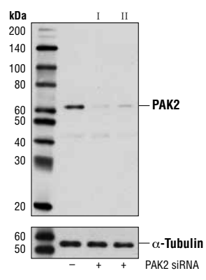
Western blot analysis of extracts from HeLa cells, transfected with 100 nM SignalSilence® Control siRNA (Unconjugated) #6568 (-), SignalSilence® PAK2 siRNA I #6467 (+) or SignalSilence® PAK2 siRNA II (+), using PAK2 (C17A10) Rabbit mAb #2615 and \alpha -Tubulin (11H10) Rabbit mAb #2125. The PAK2 (C17A10) Rabbit mAb confirms silencing of PAK2 expression, while the \alpha -Tubulin (11H10) Rabbit mAb is used as a loading control.
