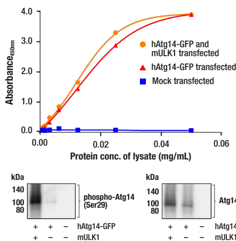
Figure 1. Co-transfection of 293T cells with constructs expressing human Atg14 and mouse ULK1 increases phosphorylation of Atg14 at Ser29 compared to cells transfected with only an Atg14 expression construct, but does not affect the level of total Atg14. Atg14 is also highly expressed in 293T cells transfected with an Atg14 expression construct compared to mock transfected cells. The relationship between lysate protein concentration from Atg14/ULK1 co-transfected, Atg14-only transfected, and mock transfected 293T cells and the absorbance at 450 nm using the PathScan® Total Atg14 Sandwich ELISA Kit #26160 is shown in the upper figure. The corresponding western blots using phospho-Atg14 (Ser29) antibody (left panel) and Atg14 antibody (right panel) are shown in the lower figure. 293T cells were co-transfected with constructs expressing GFP-tagged human Atg14 protein (hAtg14-GFP) and mouse ULK1 (mULK1), just transfected with a construct expressing GFP-tagged human Atg14 protein (hAtg14-GFP), or mock transfected, and then lysed.
