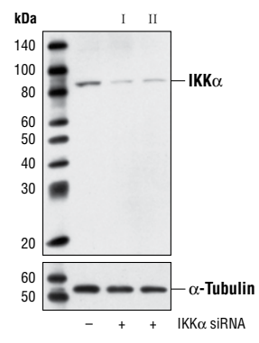
Western blot analysis of extracts from HeLa cells, transfected with 100 nM SignalSilence® Control siRNA (Unconjugated) #6568 (-), SignalSilence® IKKα siRNA I #6372 (+) or SignalSilence® IKKα siRNA II (+), using IKKα Antibody #2682 (upper) or α-Tubulin (11H10) Rabbit mAb #2125 (lower). The IKKα Antibody confirms silencing of IKKα expression, while the α-Tubulin (11H10) Rabbit mAb is used as a loading control.
