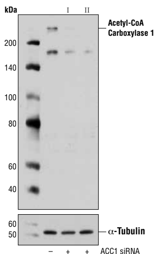
Western blot analysis of extracts from HeLa cells, transfected with 100 nM Signal Silence® Control siRNA (Unconjugated) #6568 (-), Signal Silence® Acetyl-CoA Carboxylase 1 siRNA I #6224 (+) or Signal Silence® Acetyl-CoA Carboxylase 1 siRNA II (+), using Acetyl-CoA Carboxylase 1 Antibody #4190 and \alpha -Tubulin (11H10) Rabbit mAb #2125. The Acetyl-CoA Carboxylase 1 antibody confirms silencing of Acetyl-CoA Carboxylase 1 expression while the \alpha -Tubulin (11H10) Rabbit mAb is used as a loading control.
